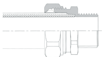
FLP Conduit with C Type fitting
